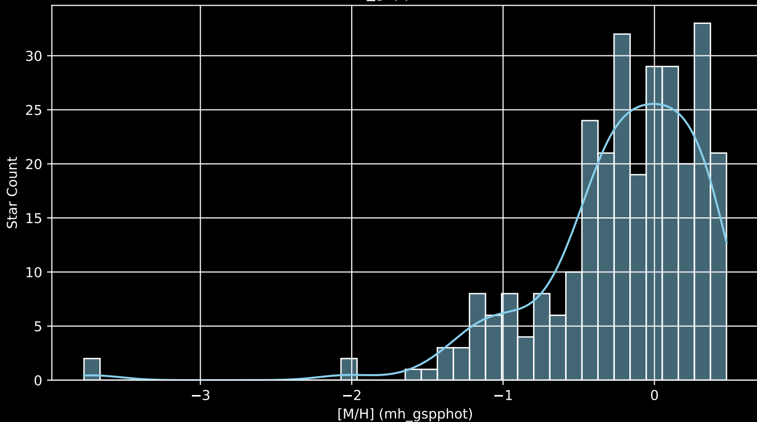
APOGEE DR17 Field: [034+00 [M/H] (mh_gspphot) (n= 290)
