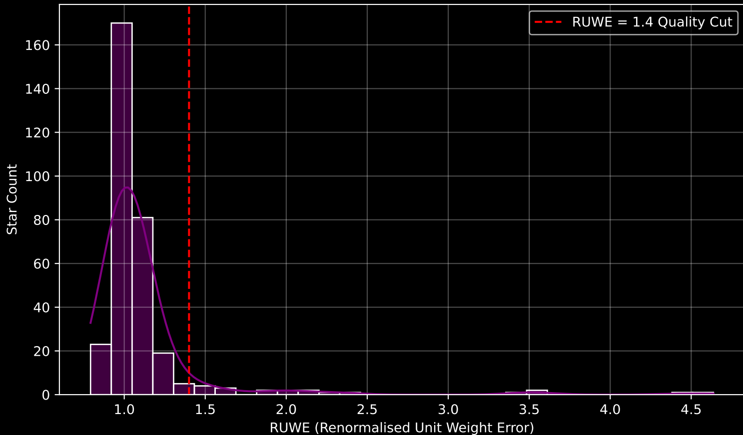
GAPOGEE DR17 Field [034+00] RUWE Distribution (n= 318)
