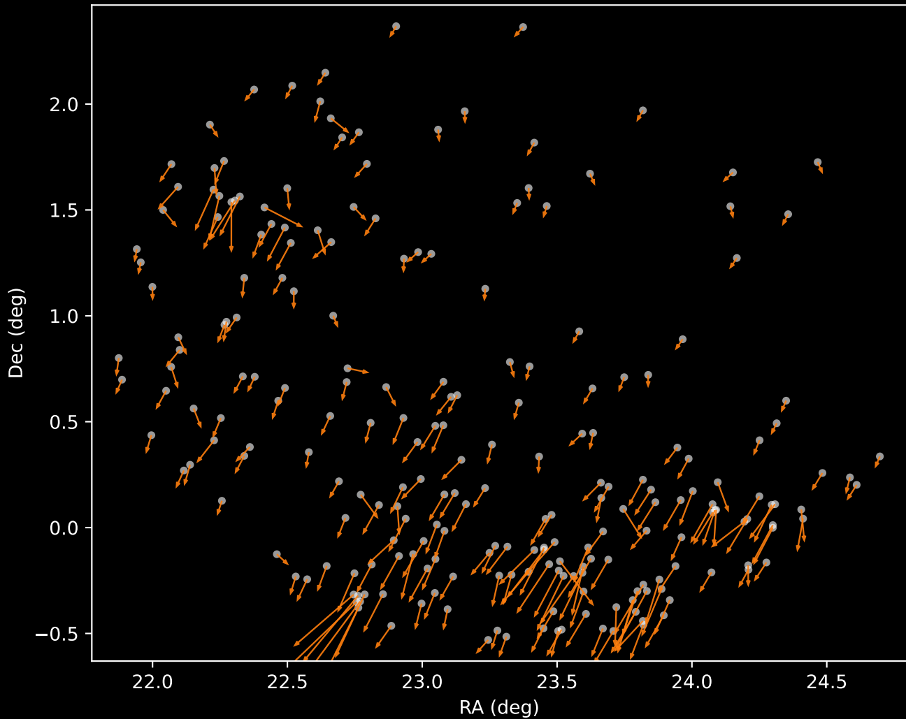
APOGEE DR17 Cluster 2 Proper Motion Vectors (n=227)
