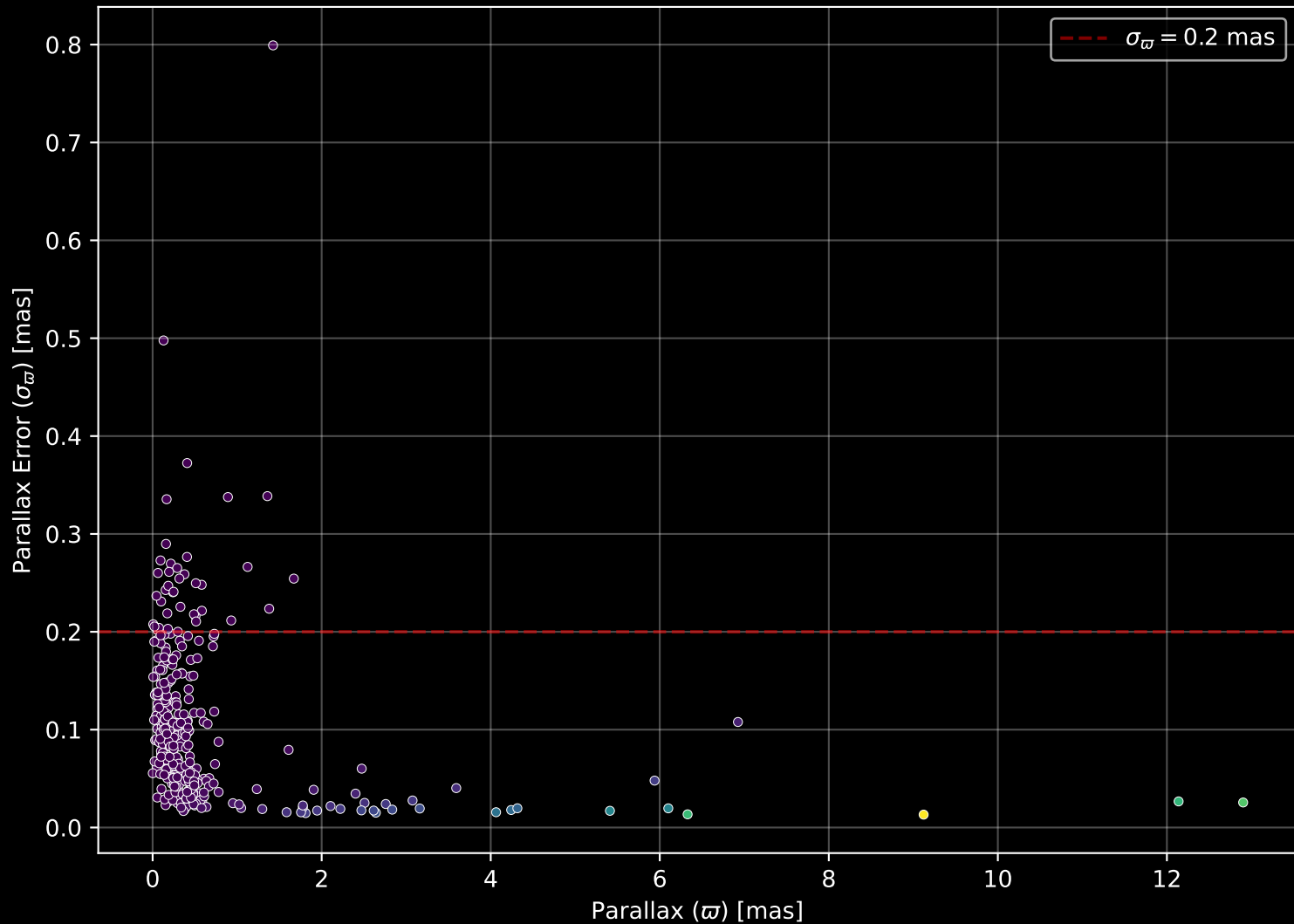
APOGEE DR17 Field: [034+00] Parallax Quality (n= 320)
