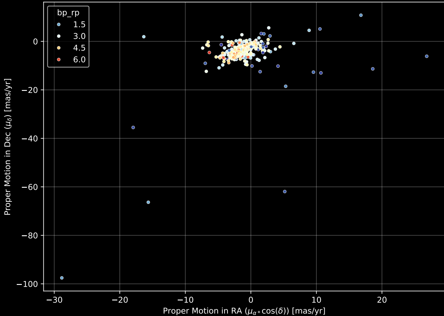
APOGEE DR17 Field: [034+00] Proper Motion Diagram (n= 320)
